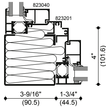
90° OUTSIDE CORNER
