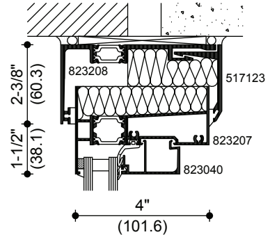
DEFLECTION HEAD [ALLOWS ± 5/8" (15.9) MOVEMENT]
