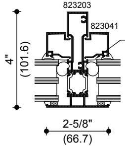
TRIPLE GLAZED [ACCEPTS 1-3/4" (44) SEALED UNITS]
